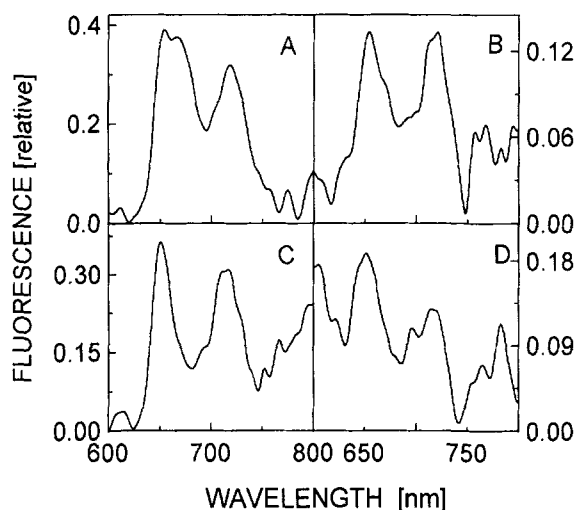
Fig. 6. Fluorescence spectra of porphyrins. TPP in PVA/chloroform; (A) \lambda_{\text{ex}} = 419 nm; (B) \lambda_{\text{ex}} = 515 nm. TPP in PMMA/chloroform; (C) \lambda_{\text{ex}} = 418 nm; (D) \lambda_{\text{ex}} = 515 nm.
